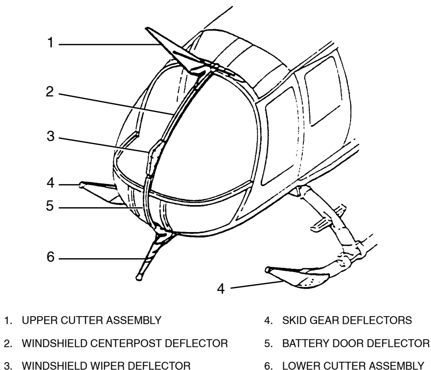
Fig. 1 Wire Strike Protection System Components
